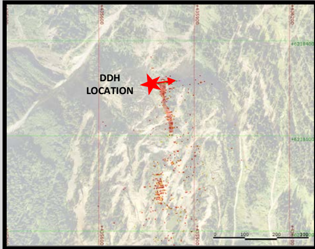
PLAN VIEW OF SILVER COIN DEPOSIT
